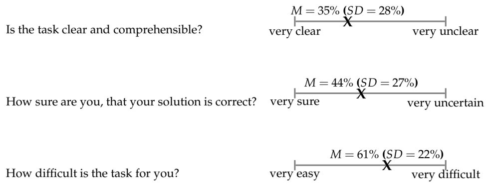
Figure 1: Mean ratings of the task comprehensibility, confidence in correctness, and difficulty (Experiment 1, N_1 = 141 ).
