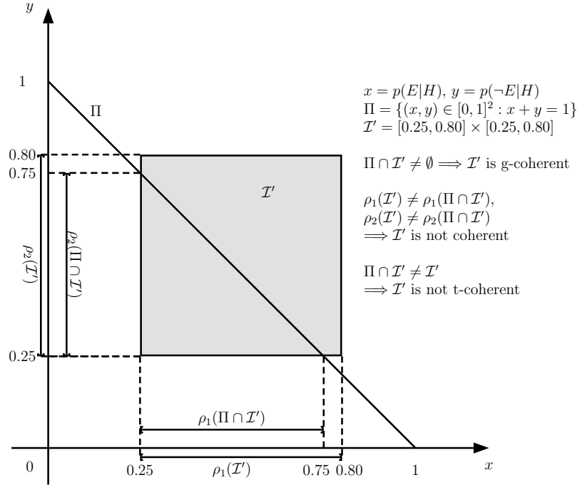
Figure 1: The g-coherent assessment \mathcal{I}' on (E|H, -E|H) explained in Example 1.
