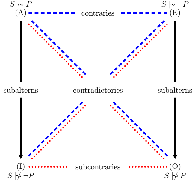
Figure 4: Default square of opposition defined on the four sentence types introduced in Table 1. It provides a new interpretation of the traditional square of opposition (see, e.g., [33]), where the corners are labeled by “Every S is P ” (A), “No S is P ” (E), “Some S is P ” (I), and “Some S is not P ” (O).
